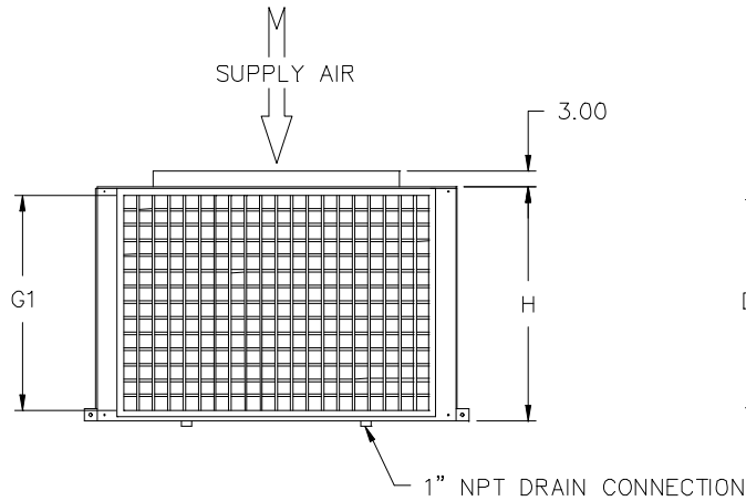
ELEVATION VIEW
